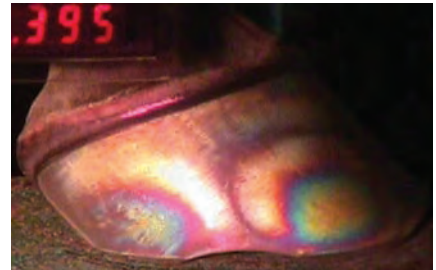
An isochromatic fringe pattern from photoelastic coating experiments to determine effects on the stress state in equine hooves resulting from different trim practices by farriers. Crippling diseases such as laminitis are related to hoof stress. Photo courtesy of Dr. Loic Dejardin, DVM, of the College of Veterinary Medicine, Michigan State University.
